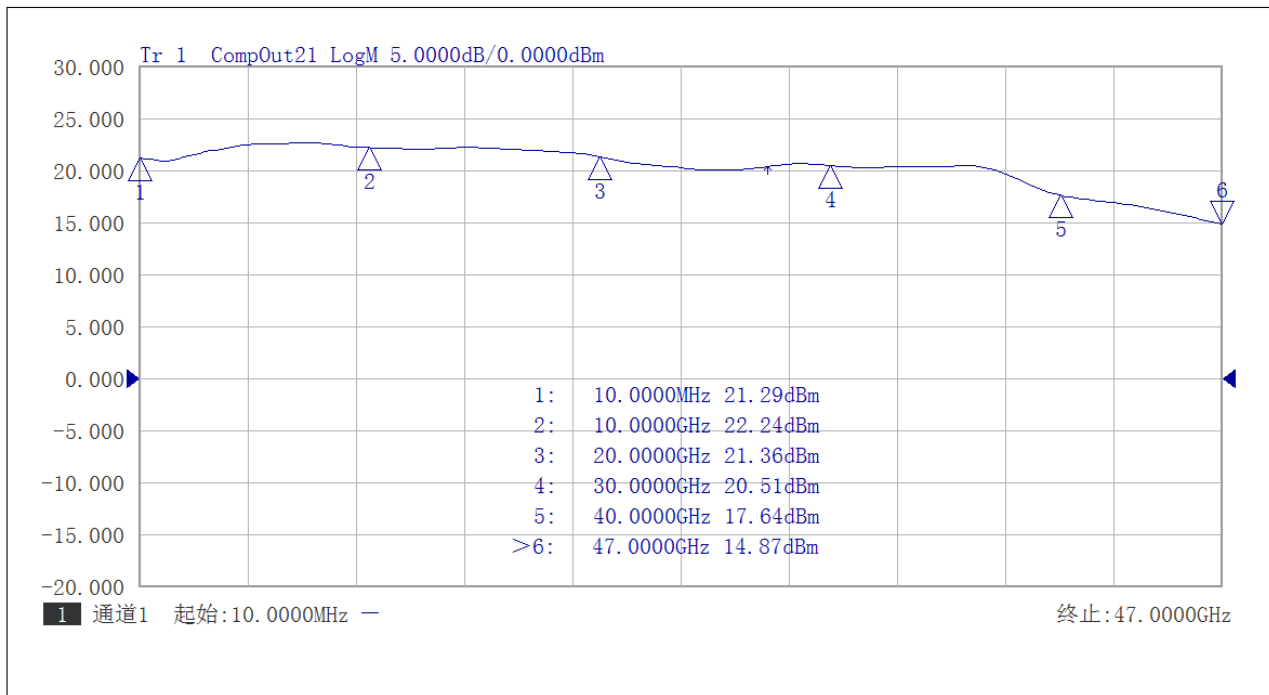
P1 vs Frequency 10MHz-50GHz
