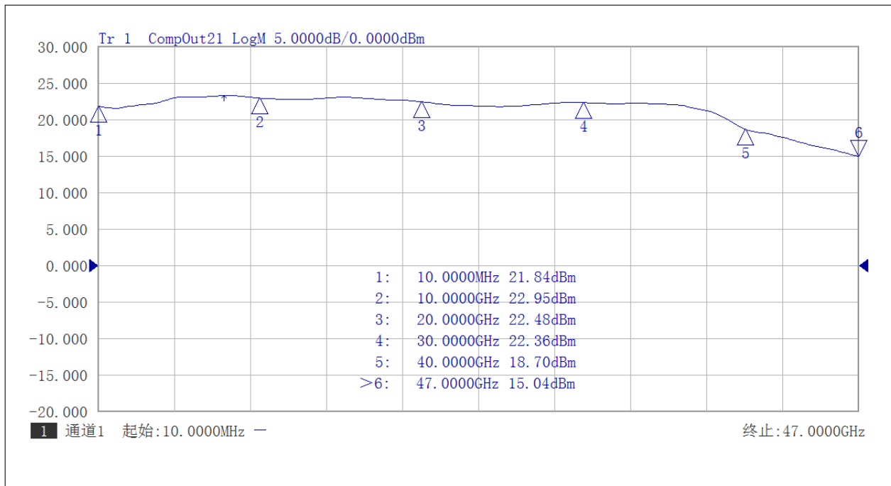
P3 vs Frequency 10MHz-50GHz
